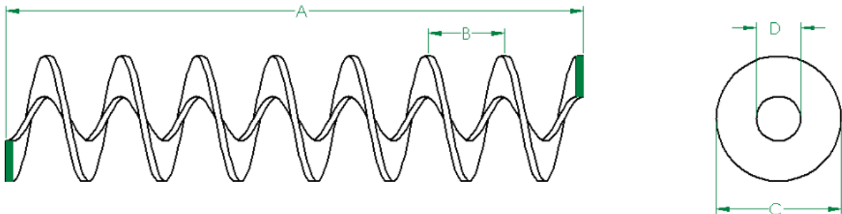
HELICOID FLIGHTING
